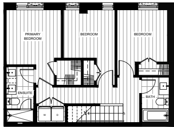
LEVEL 3
