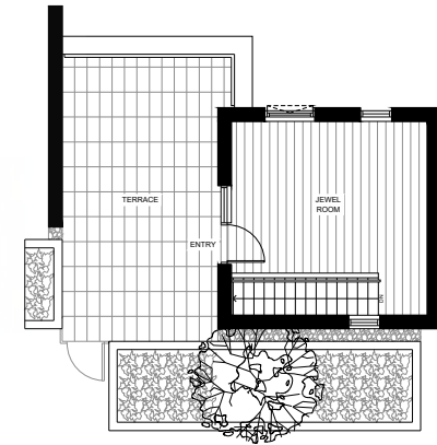
LEVEL 5
