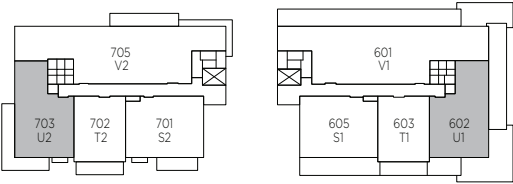
NORTH PENTHOUSE LEVEL / SOUTH LEVEL 6
