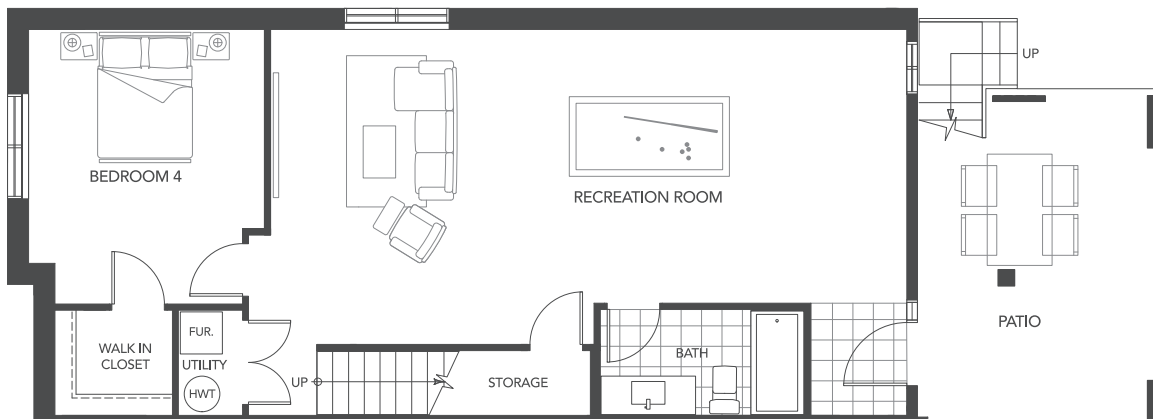
LOWER 844 SQ.FT.
