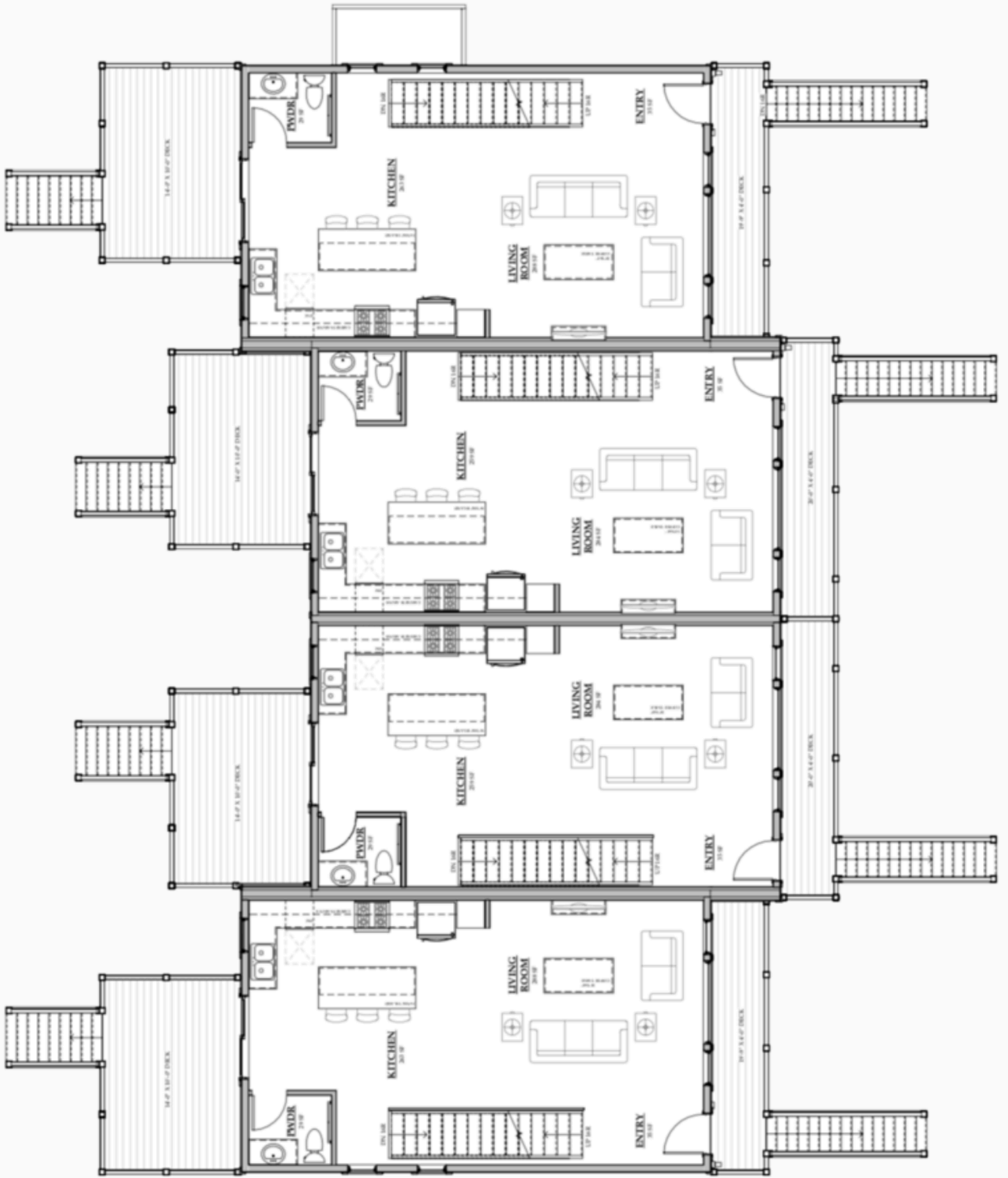
Granite Heights Luxury Townhome Development: Main Floor Plan
