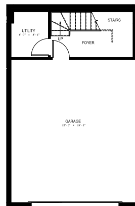
Garage - 750 Sq.Ft.
