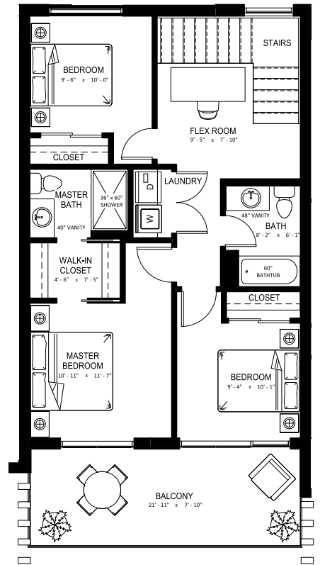
Second Floor - 753 Sq.Ft.
