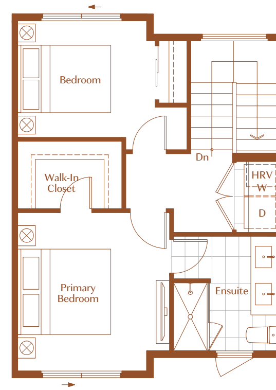
UPPER LEVEL
