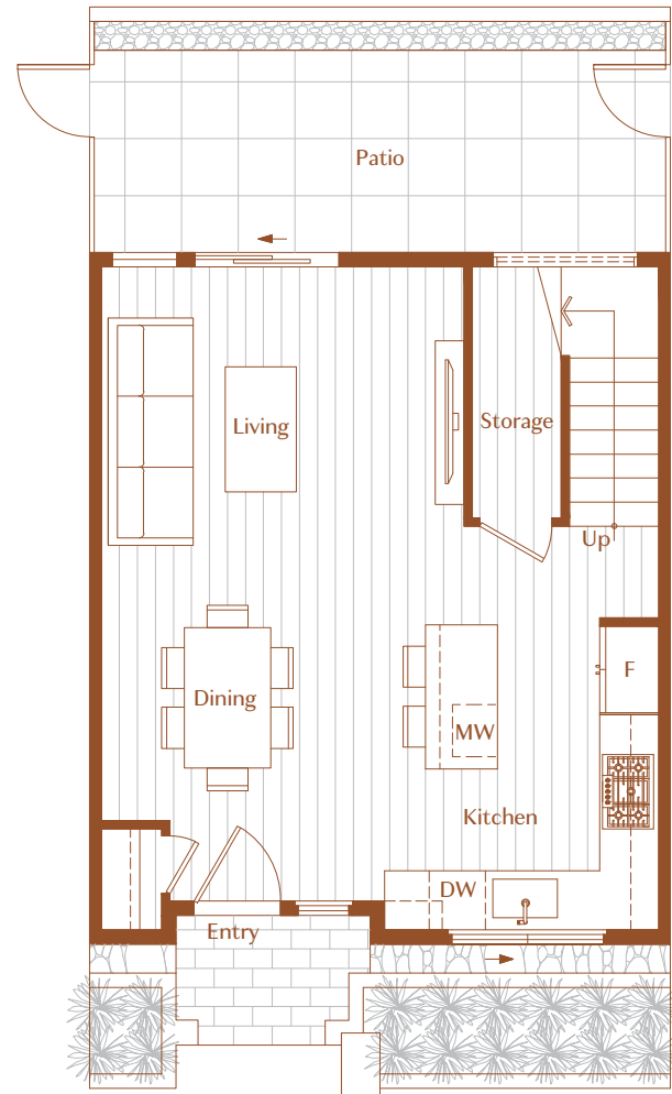
MAIN LEVEL
