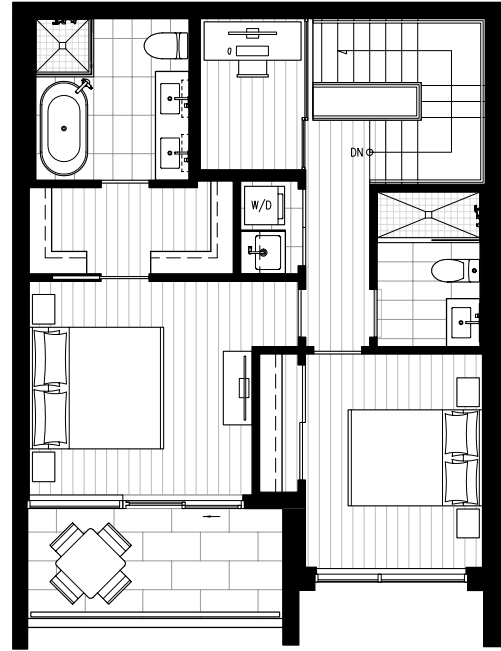
Upper Level
