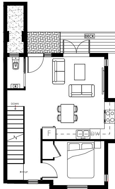
MAIN FLOOR 502 sq. ft.
