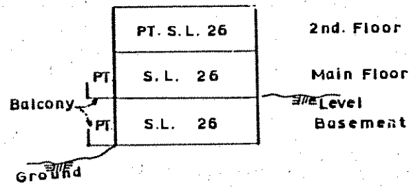
SECTION 'S'-S'
