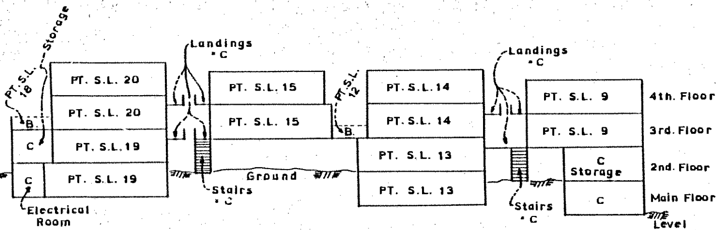
SECTION 'I-I'
