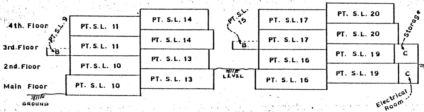
SECTION 'K'-'K'
