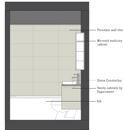
BATHROOM ELEVATION B
