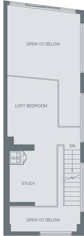
UPPER FLOOR
