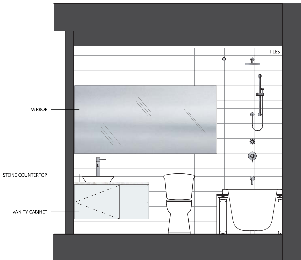
ELEVATION C
