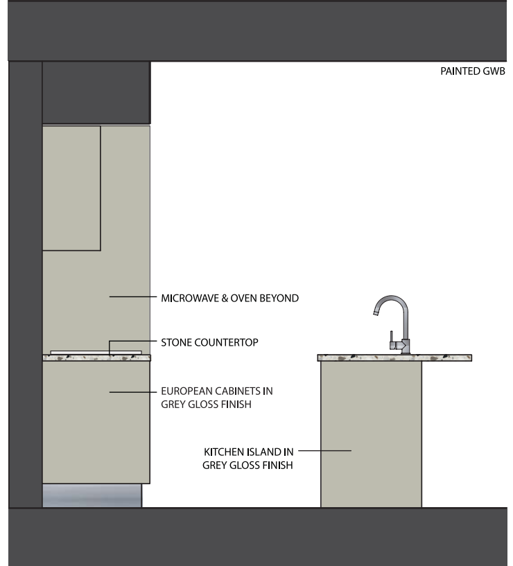
ELEVATION C
