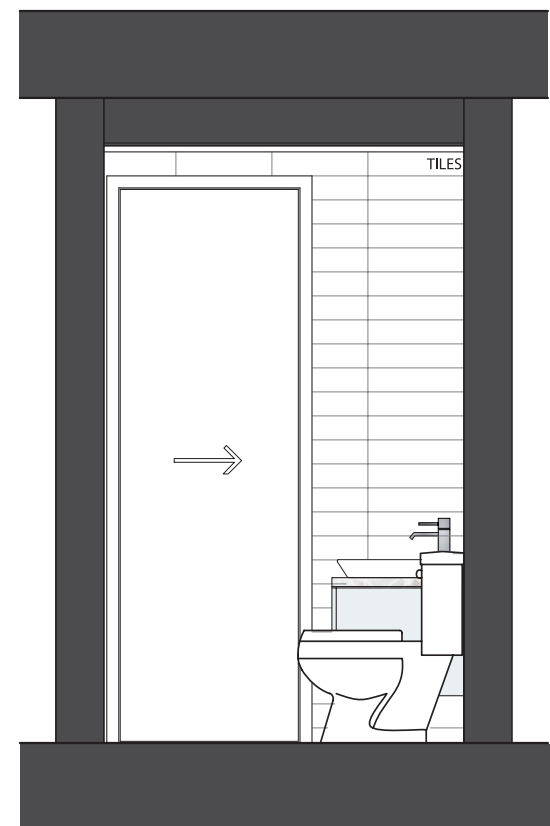
ELEVATION D
