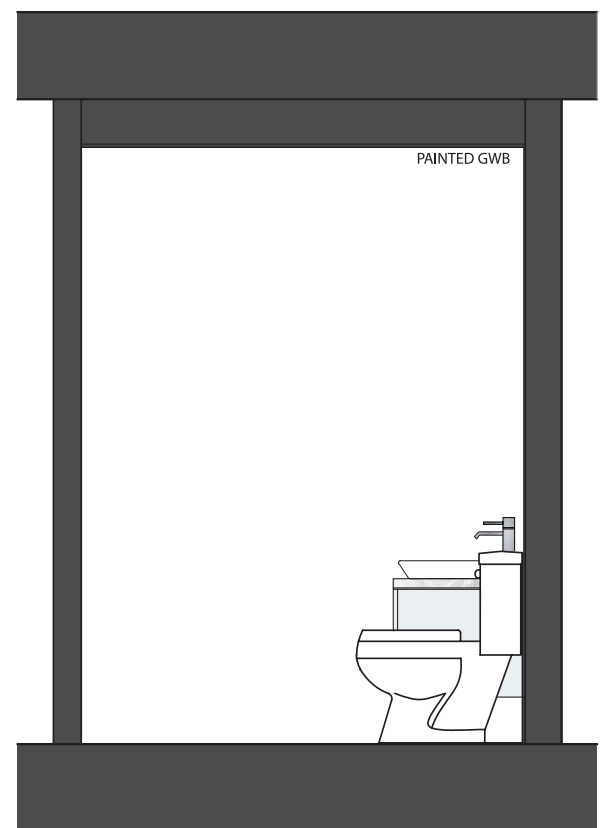
ELEVATION D
