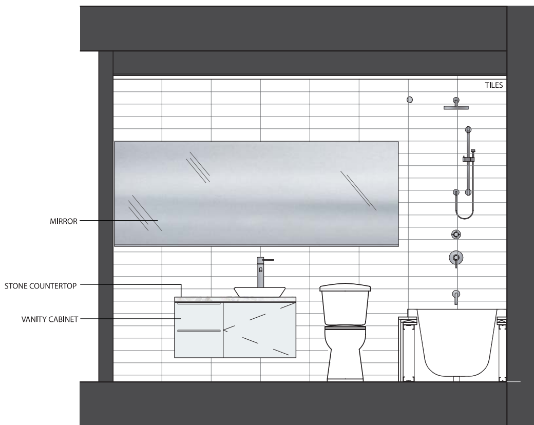
ELEVATION C
