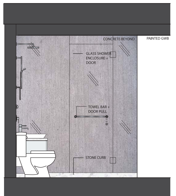
ELEVATION D
