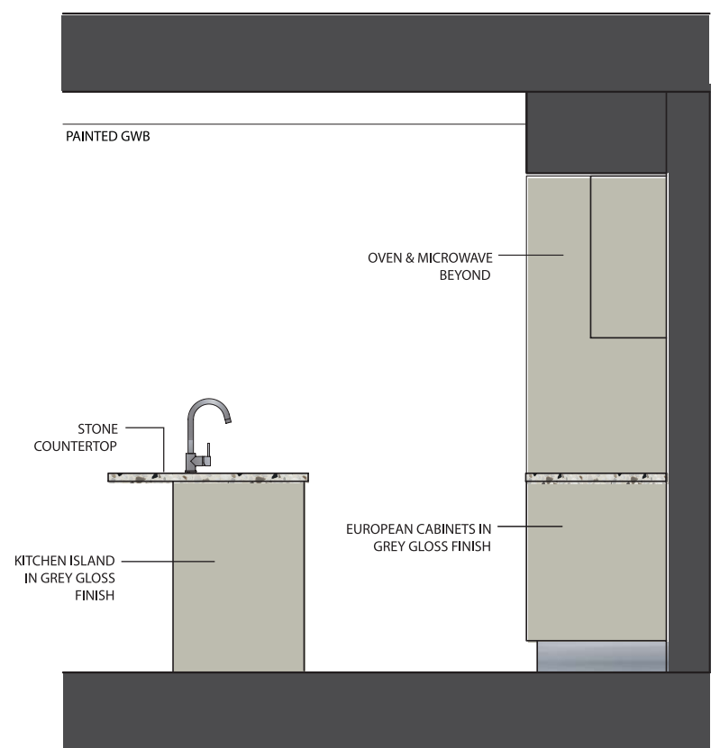
ELEVATION C
