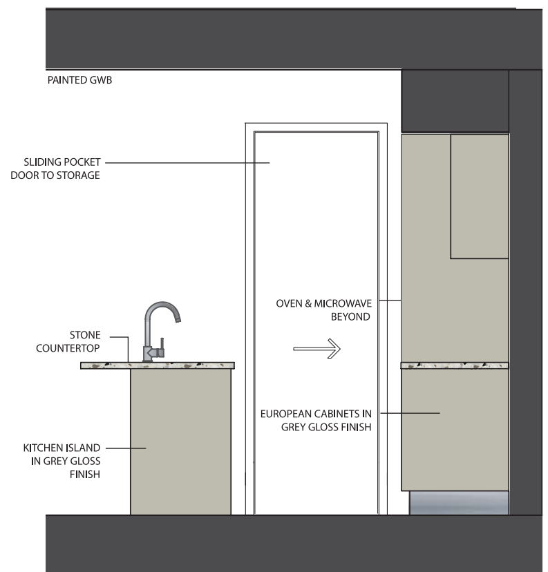
ELEVATION C
