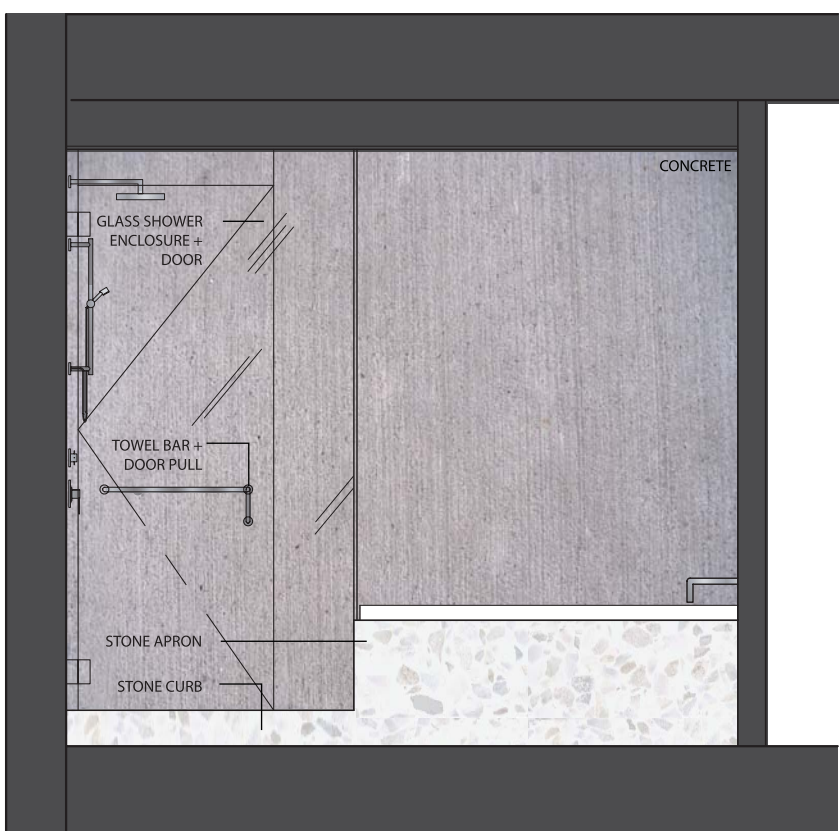
ELEVATION C
