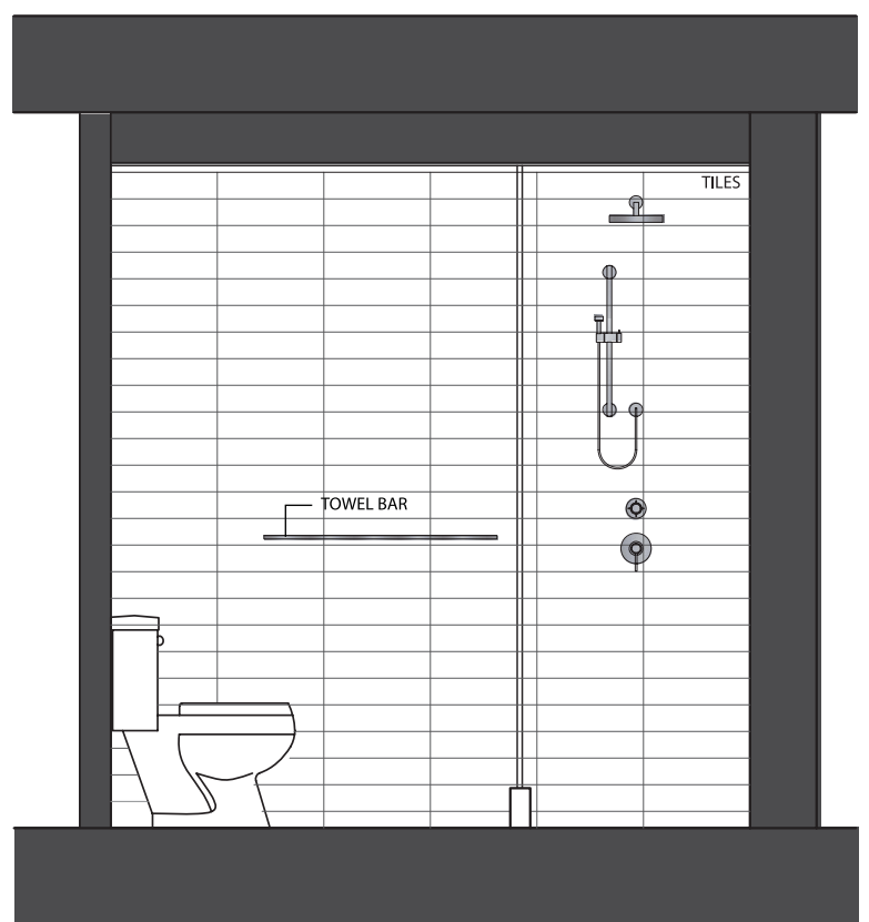
ELEVATION D
