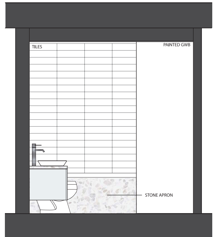
ELEVATION D
