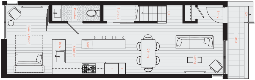
LEVEL 2
