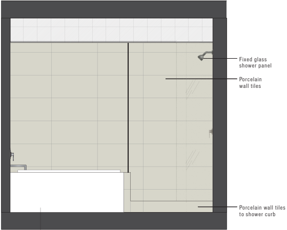
BATHROOM ELEVATION B
