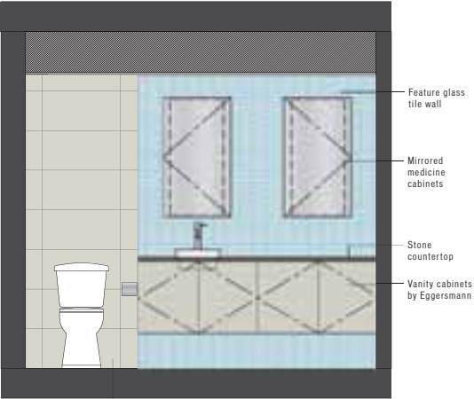
BATHROOM ELEVATION A
