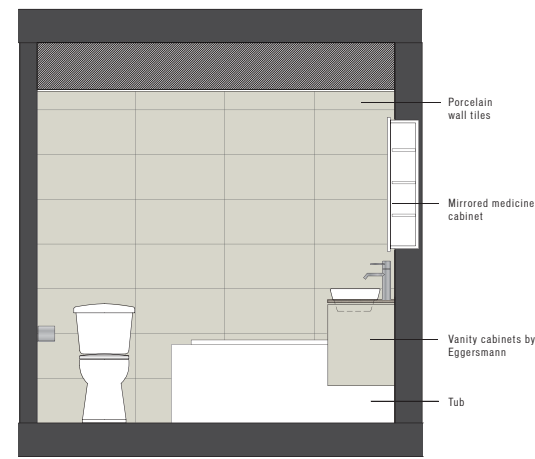
BATHROOM ELEVATION B
