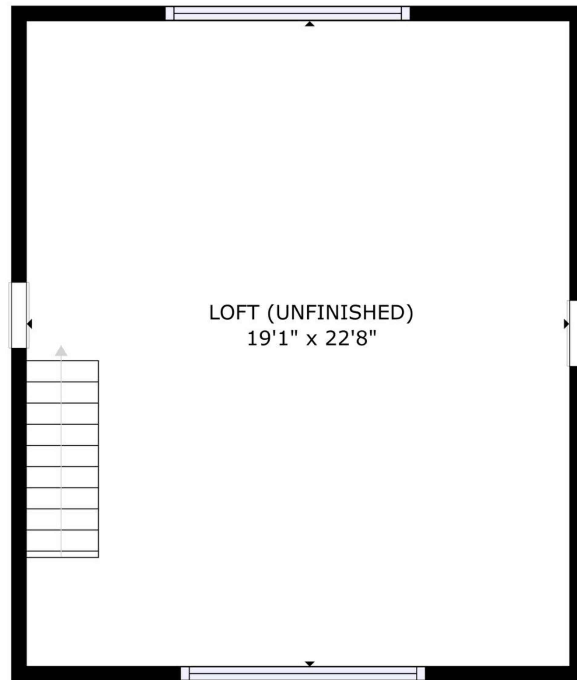
Upper Level - 433 sq.ft Ceiling Height: 8'0"
