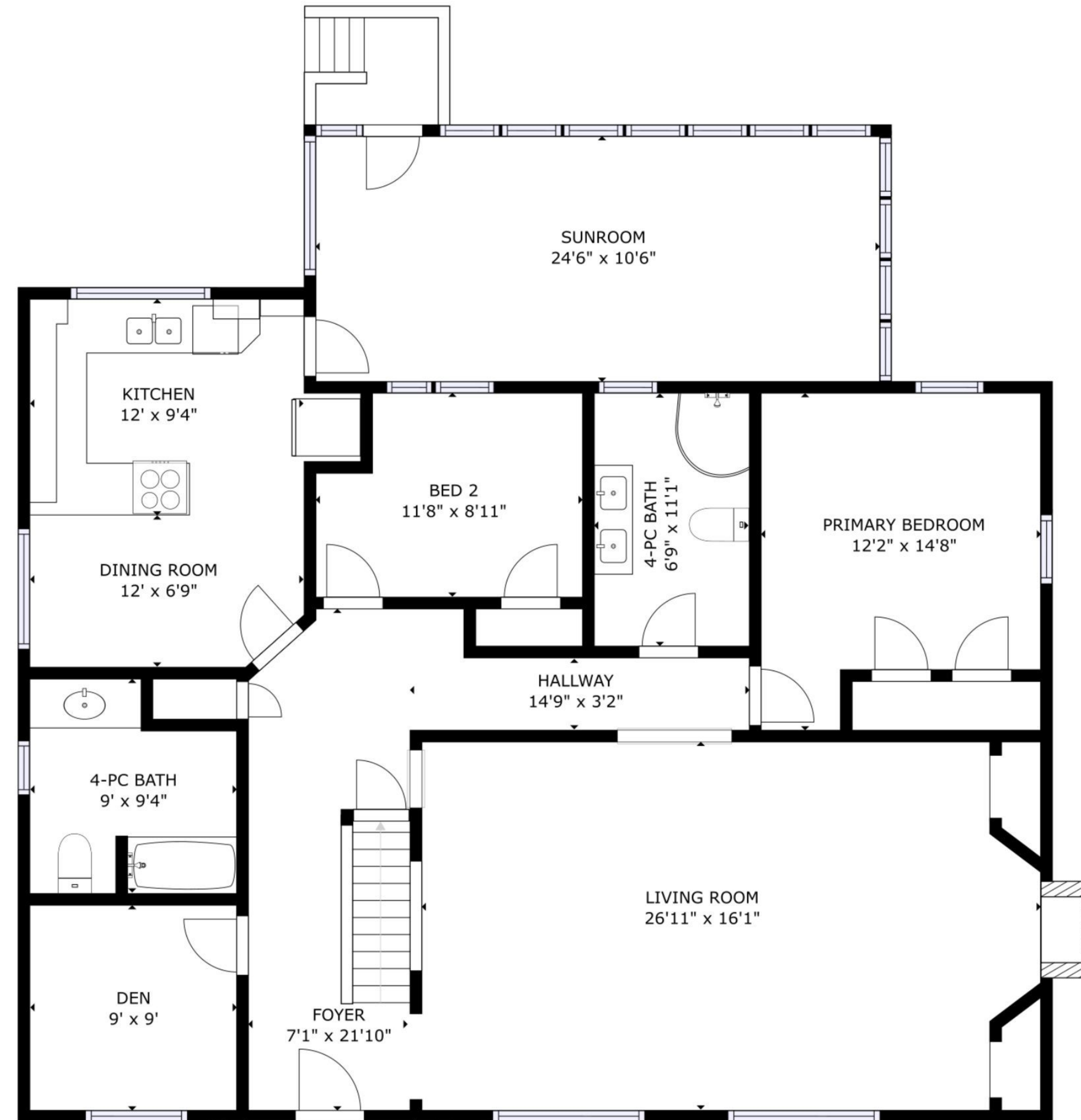
Main Floor - 1,701 sq.ft Ceiling Height: 9'04"
