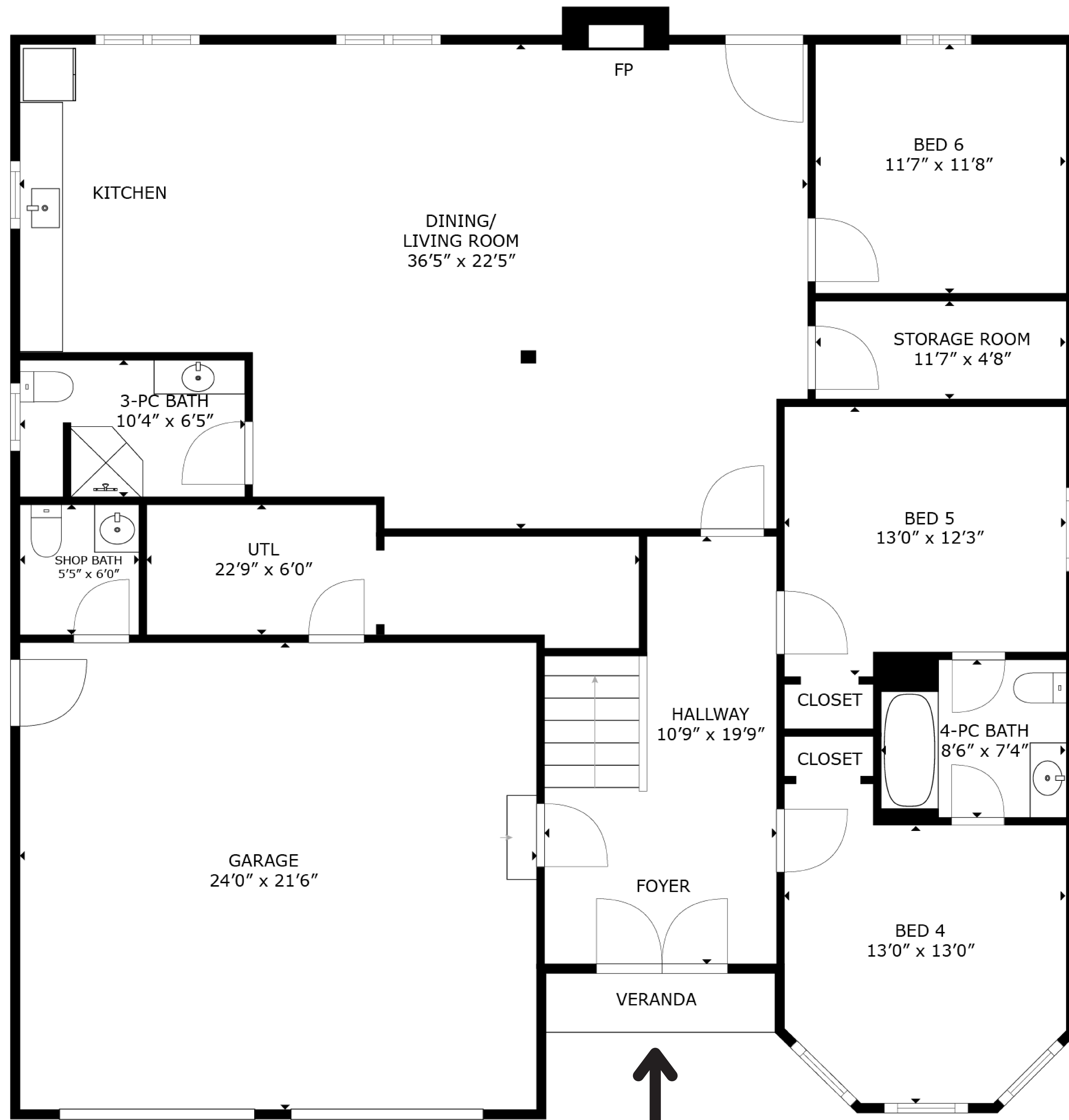
First Floor - 1,766 sq.ft Ceiling Height: 8'93"
