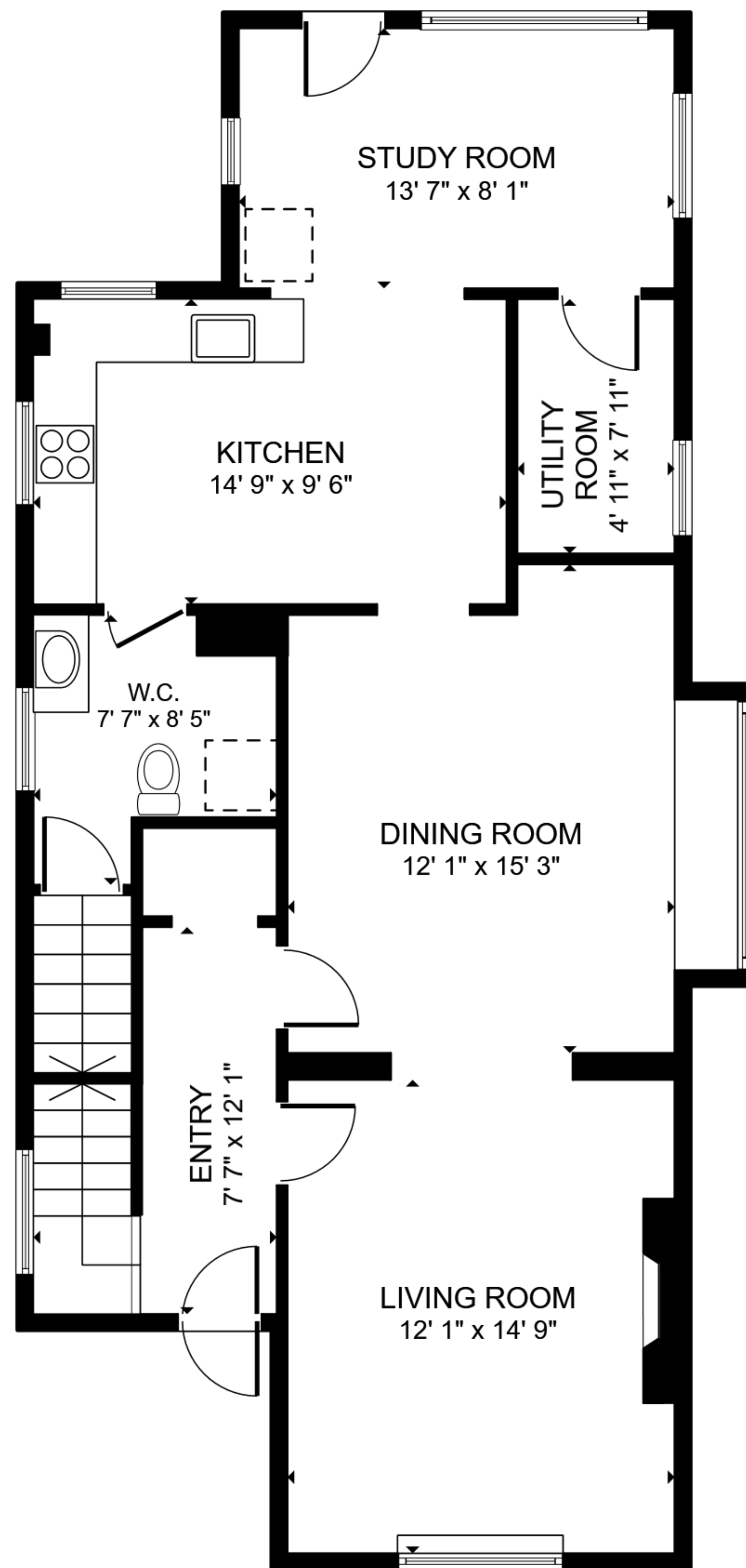
FLOOR 2
