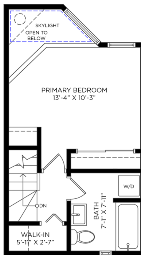
UPPER FLOOR - 302 SQ.FT. CEILING HEIGHT: 8'-0"
