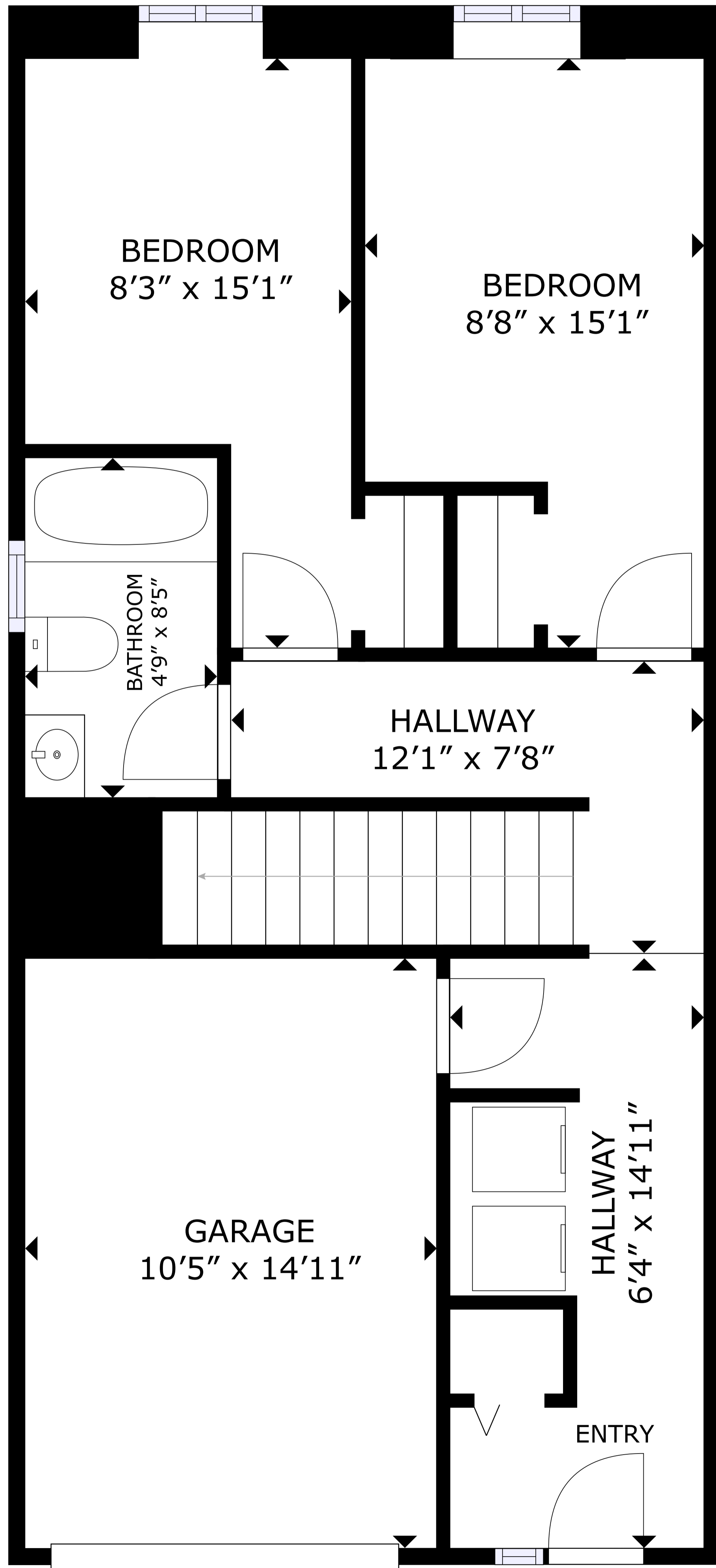
1ST FLOOR
