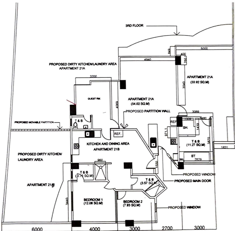
LAY-OUT PLAN OF CONDO UNIT 21A/B LOCATION: EGI MARIBAGO LLC
