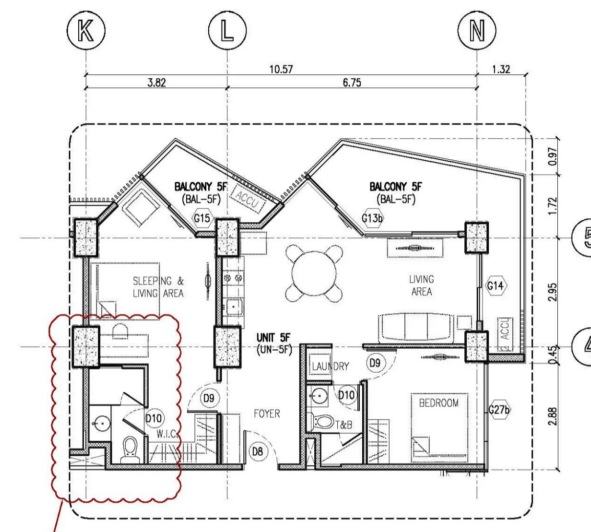
TAMBULLI - RESIDENTIAL TOWER F 8TH, 10TH, 11TH, 12TH, 13TH, 14TH, 15TH, 16TH 17TH & 18TH FLOOR PLAN SCALE 1 : 100 METERS 0 0.5 1 2 5
