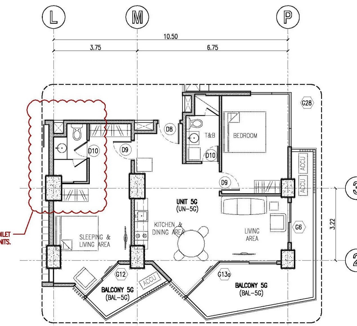
CLARIFICATION ON TOILET LAYOUT FOR 2BR UNITS.
