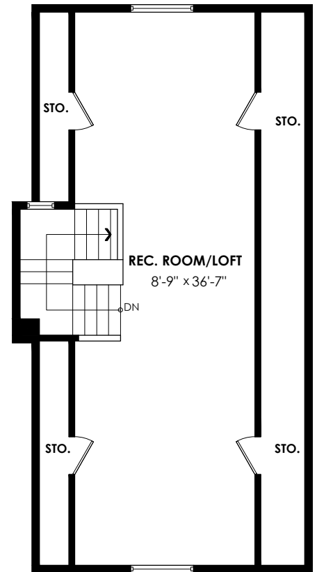
Upper Floor Plan Floor Area: 710 sq.ft. Ceiling Height: 7'
