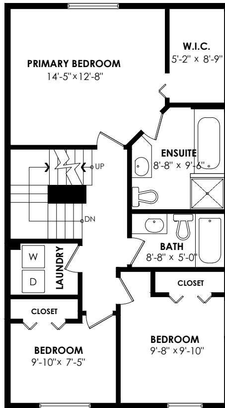
1st Floor Plan Floor Area: 785 sq.ft. Ceiling Height: 8'-1"
