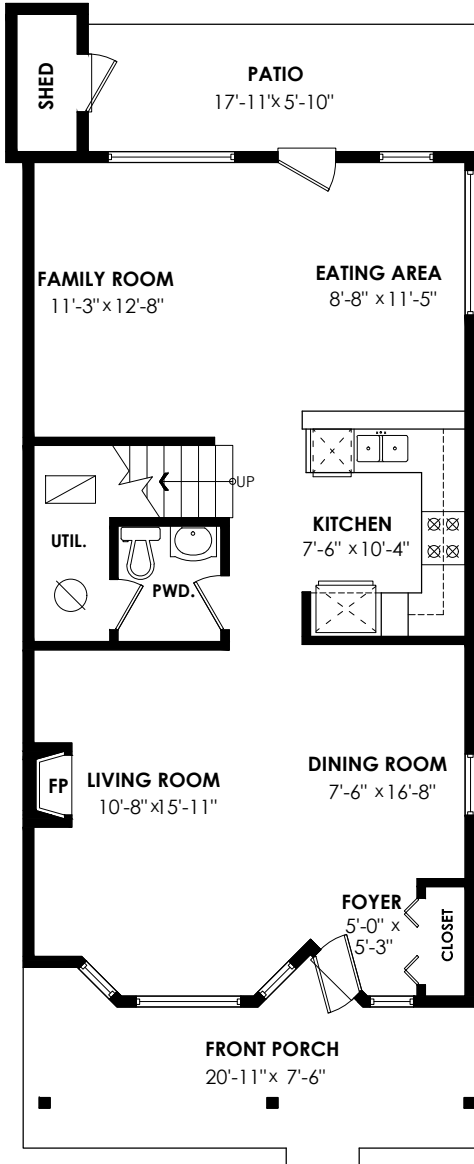
Main Floor Plan Floor Area: 811 sq.ft. Ceiling Height: 9'
