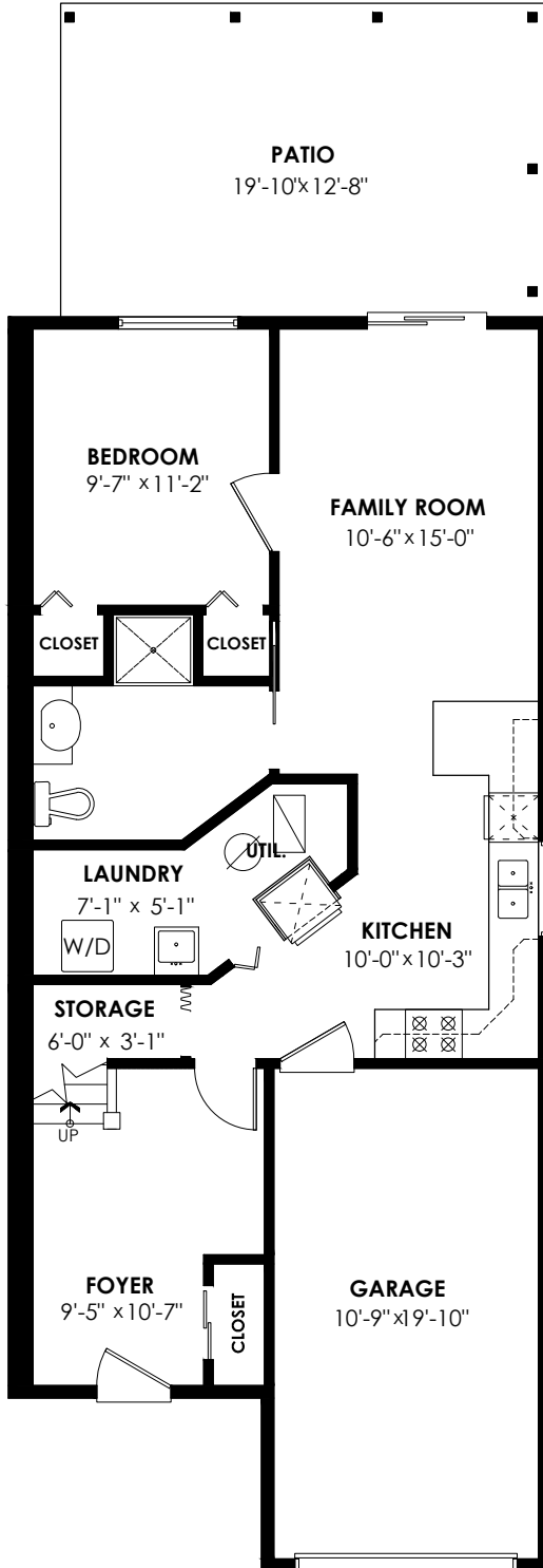
Lower Floor Plan Floor Area: 788 sq.ft. Ceiling Height: 8'-2"
