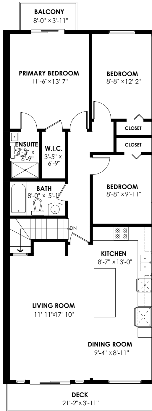
Main Floor Plan Floor Area: 1088 sq.ft. Ceiling Height: 8'-1"
