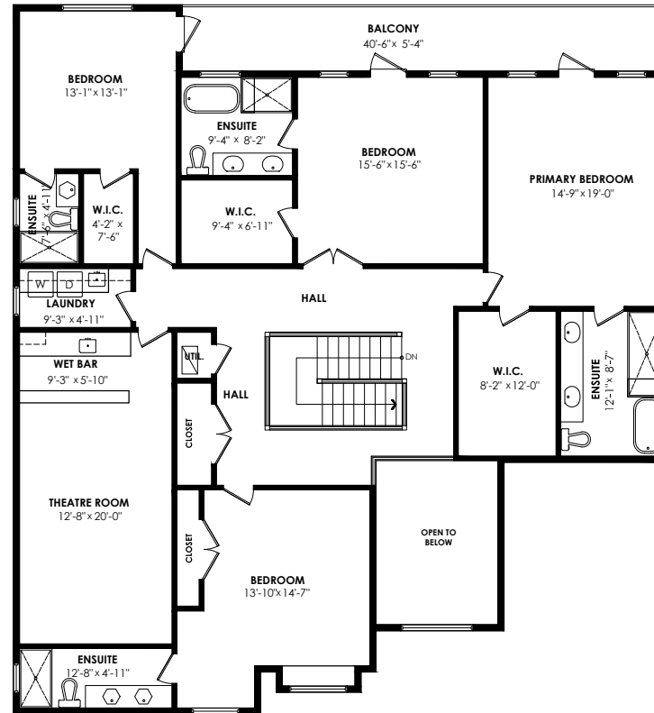
Upper Floor Plan Floor Area: 2447 sq.ft. Ceiling Height: 9'-11"
