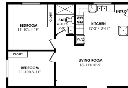
Suite Floor Plan Floor Area: 711 sq.ft. Ceiling Height: 9'
