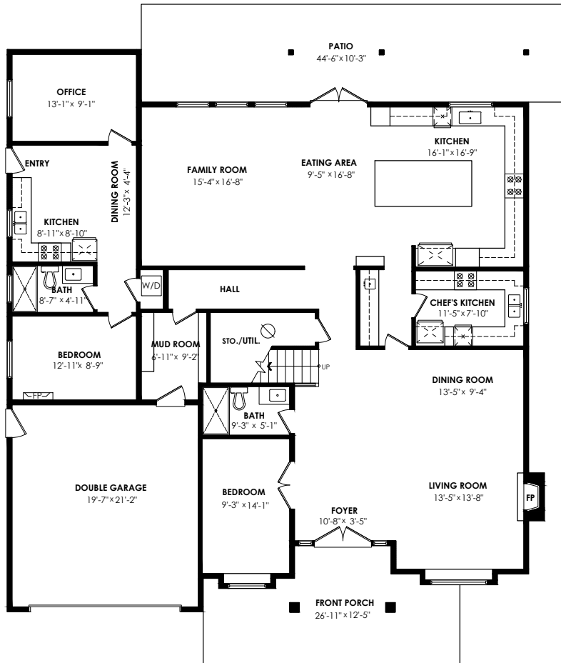
Main Floor Plan Floor Area: 2398 sq.ft. Ceiling Height: 9'-11"
