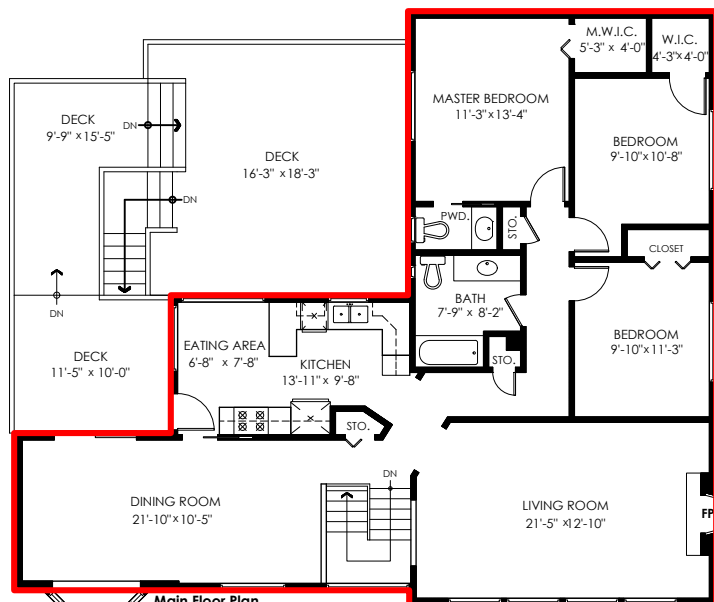
Main Floor Plan Floor Area: 1475 sq.ft. Ceiling Height: 8'-11"
