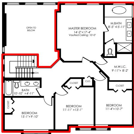
Upper Floor Plan Floor Area: 1291 sq.ft. Ceiling Height: 8'
