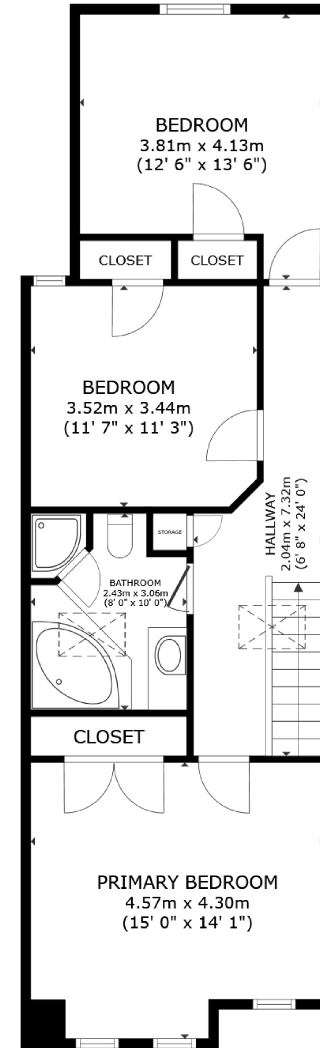
FLOOR 3
