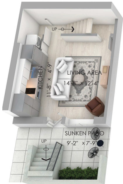
Basement Floor: 326 Sq.Ft. Ceiling Height: 8'-0"
