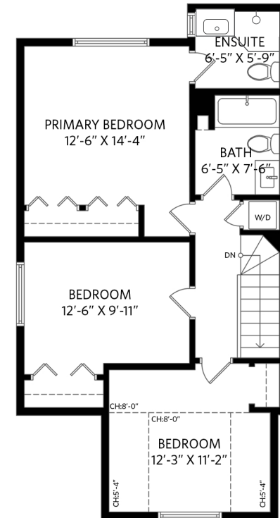
Upper Floor - 705 sq.ft. Ceiling height - 5' 4" to 8' 0"
