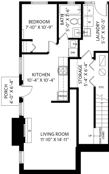
Lower Floor - 749 sq.ft. Ceiling height - 8' 0"
