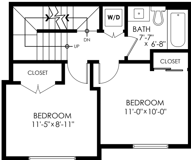
Upper Floor Plan Floor Area: 441 sq.ft. Ceiling Height: 7'-11"
