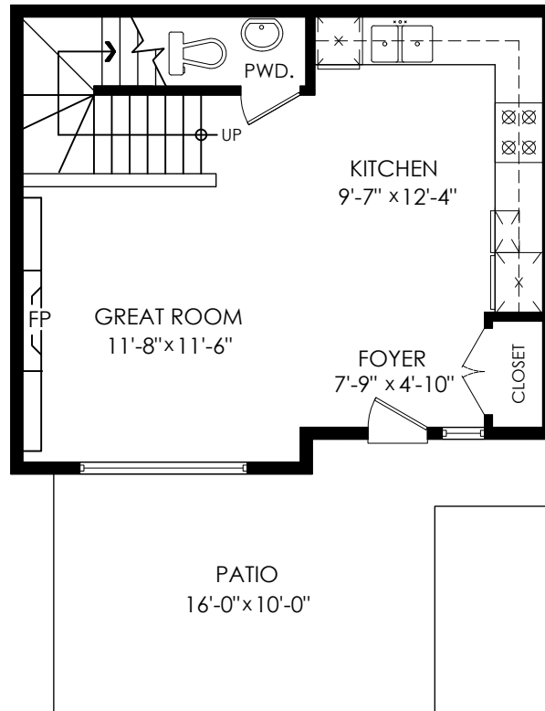
Main Floor Plan Floor Area: 434 sq.ft. Ceiling Height: 8'-11"
