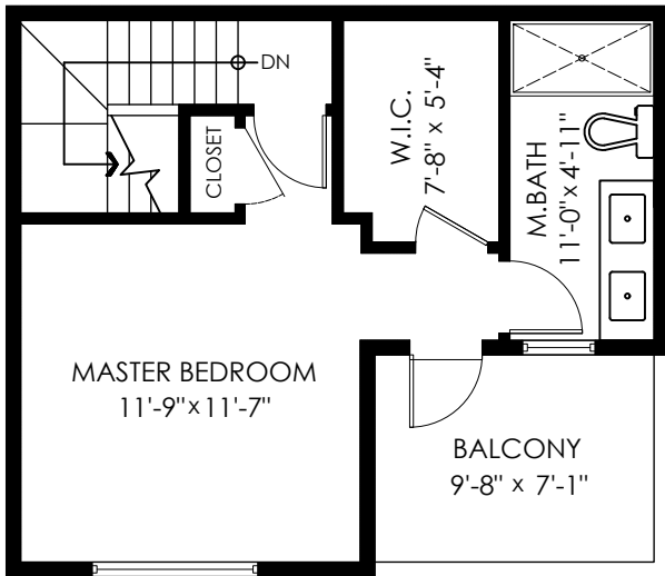
Top Floor Plan Floor Area: 372 sq.ft. Ceiling Height: 9'
