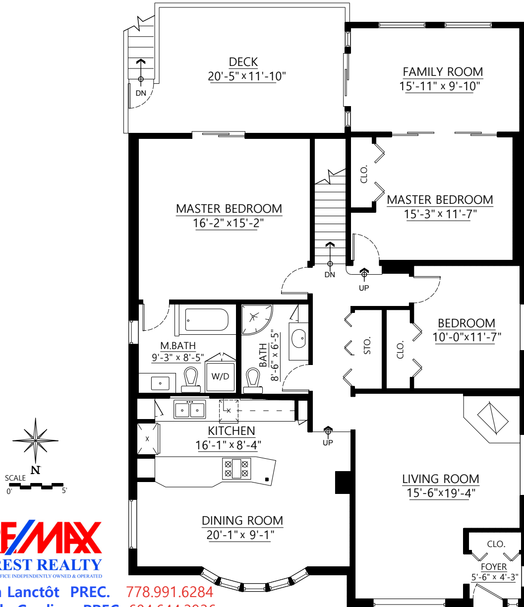
Main Floor Plan Floor Area: 1,811 sq.ft.
