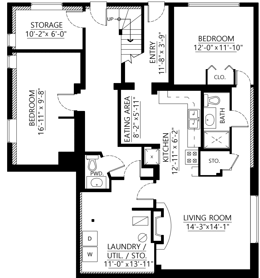
Lower Floor Plan Floor Area: 1,399 sq.ft.
