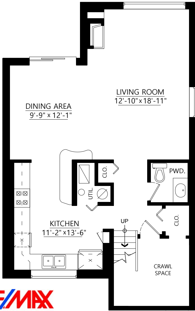
Main Floor Plan Floor Area: 738 sq.ft.
