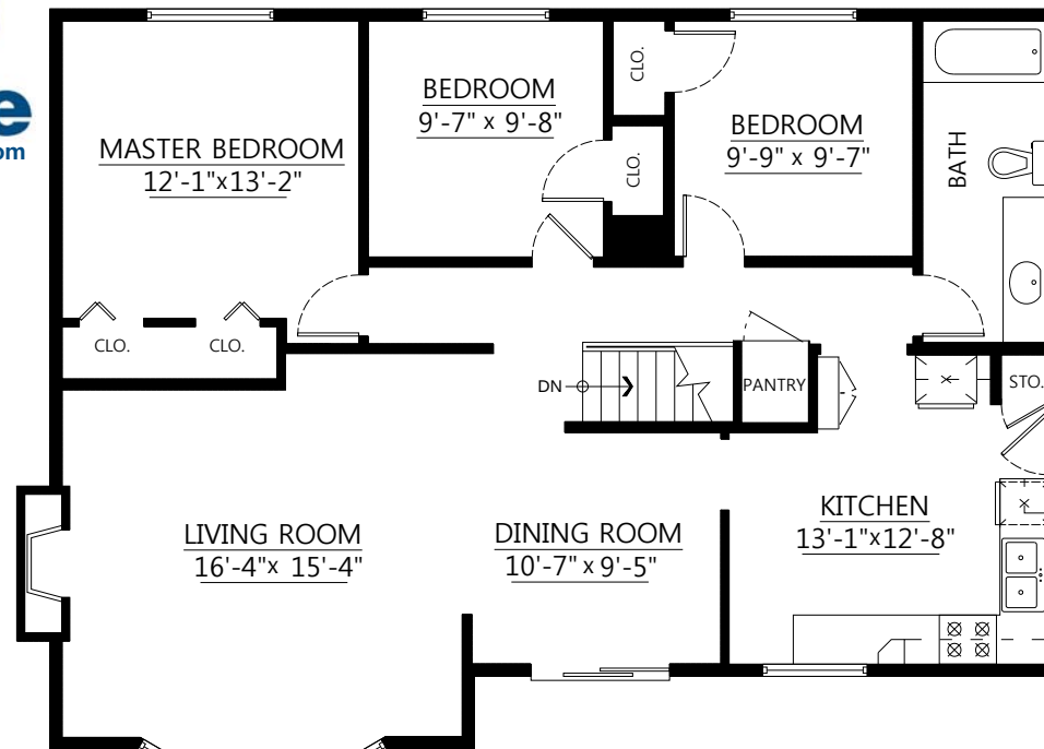
Main Floor Plan Floor Area: 1,187 sq.ft.
