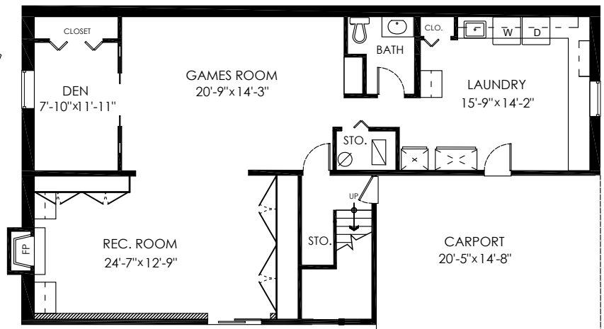
Lower Floor Plan Floor Area: 1310 sq.ft.
