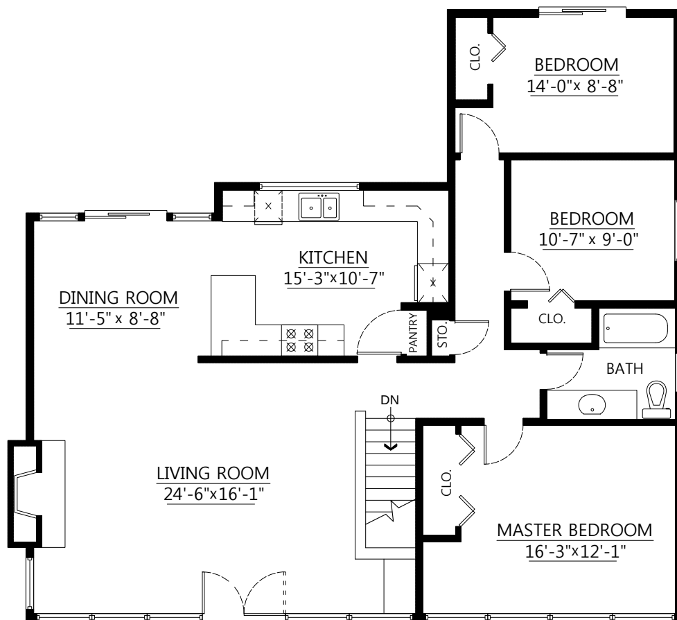
Main Floor Plan Floor Area: 1,330 sq.ft.
