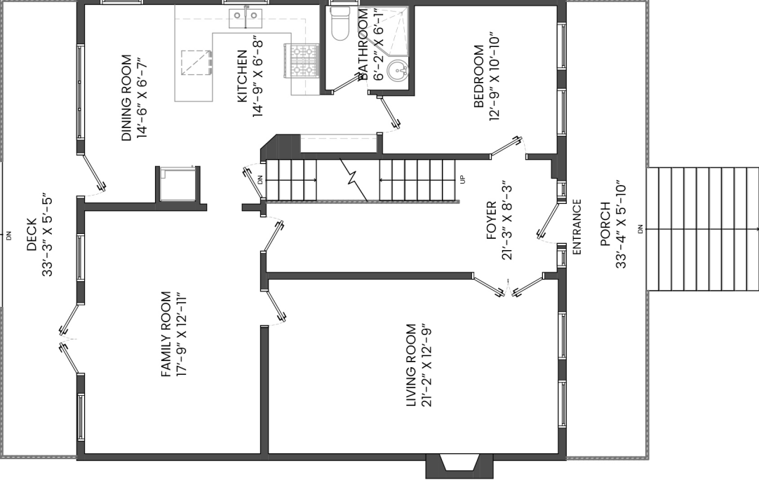
MAIN FLOOR PLAN Ceiling Height: 9'-0"
