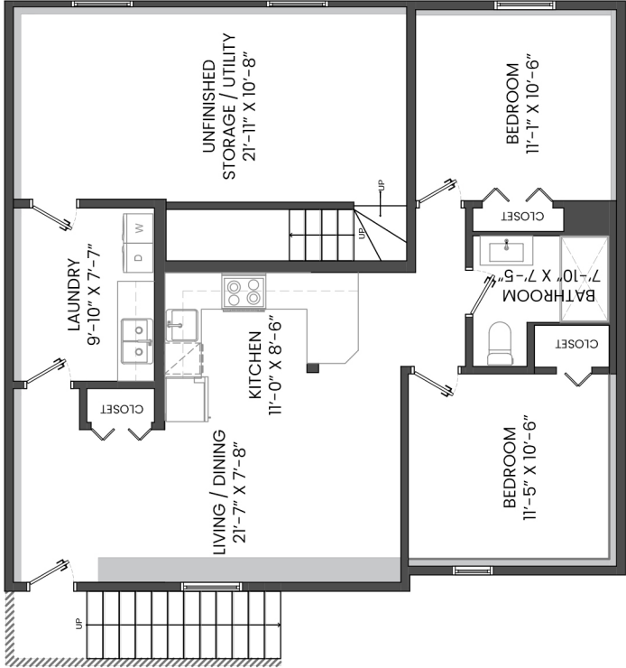
LOWER FLOOR PLAN Ceiling Height: 7'-6"
