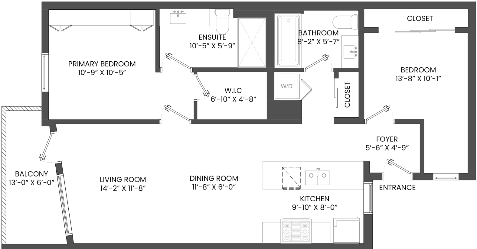
MAIN FLOOR PLAN Ceiling Height: 11'-5"
