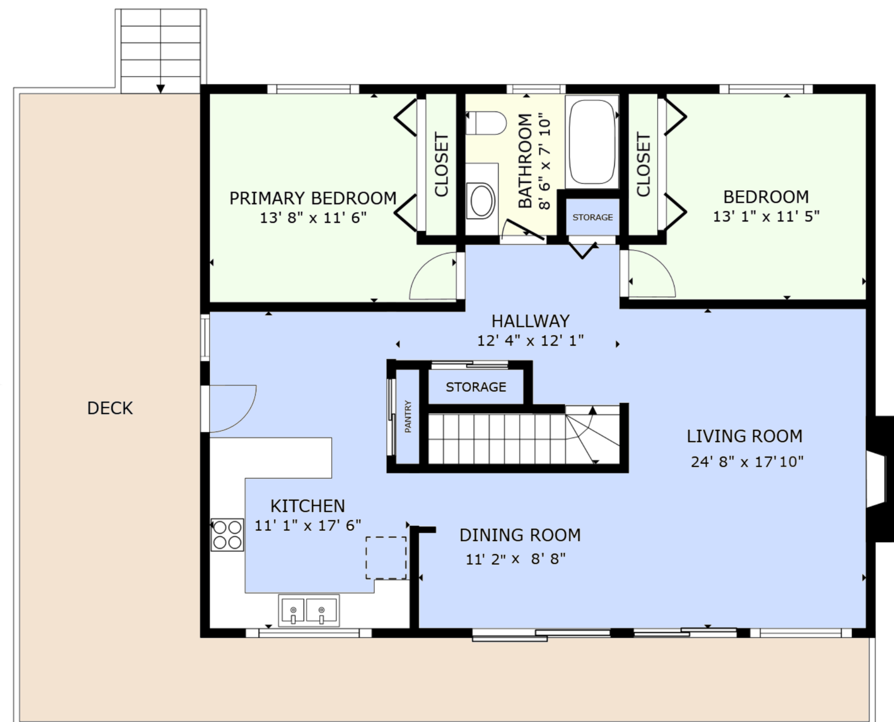
FLOOR 2
