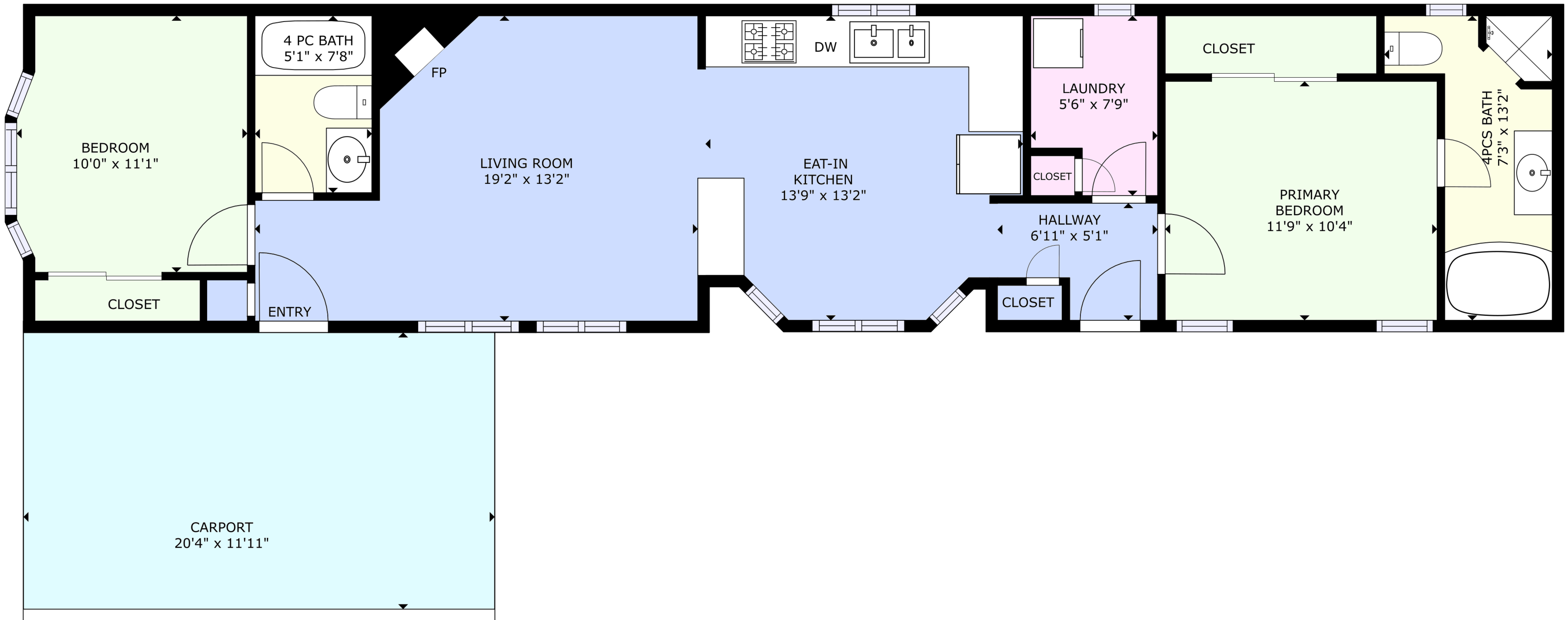
FLOOR PLAN
