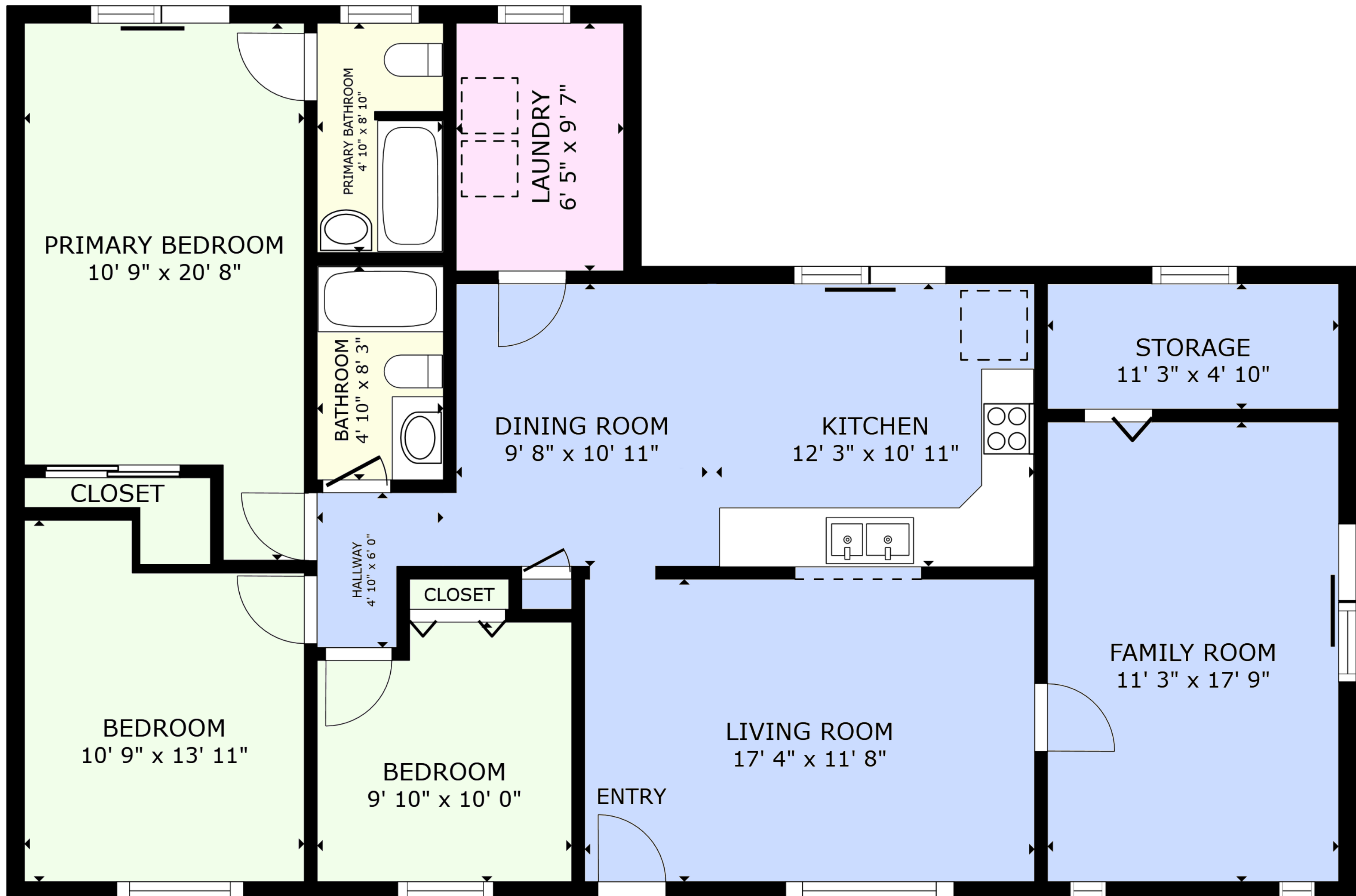
FLOOR PLAN
