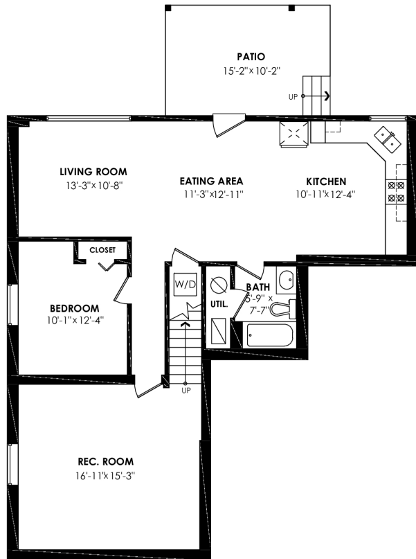
Lower Floor Plan Floor Area: 1110 sq.ft. Ceiling Height: 7'-10"
