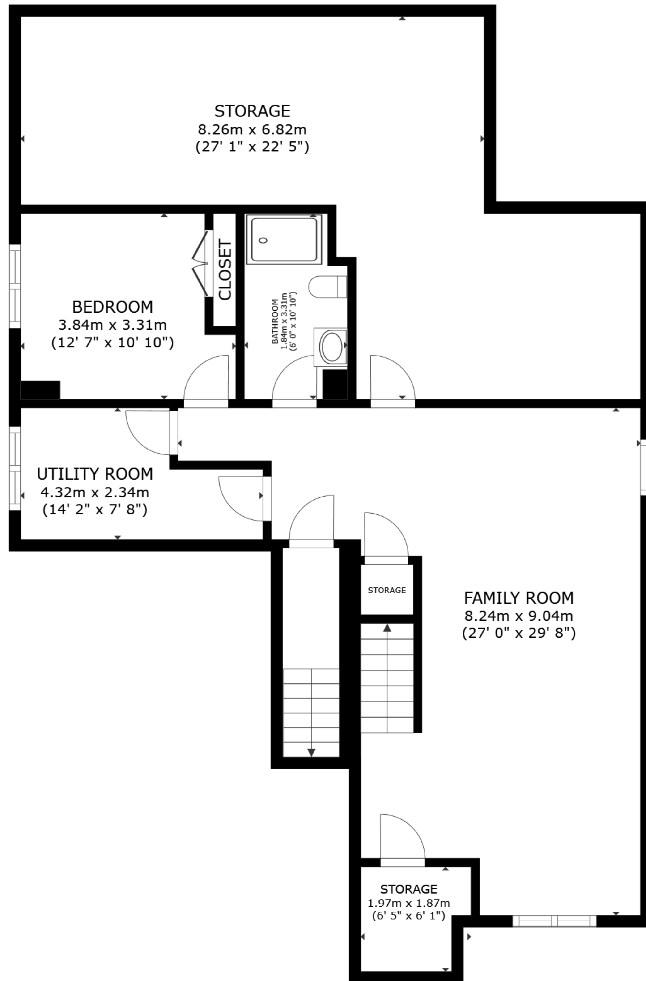
BASEMENT
