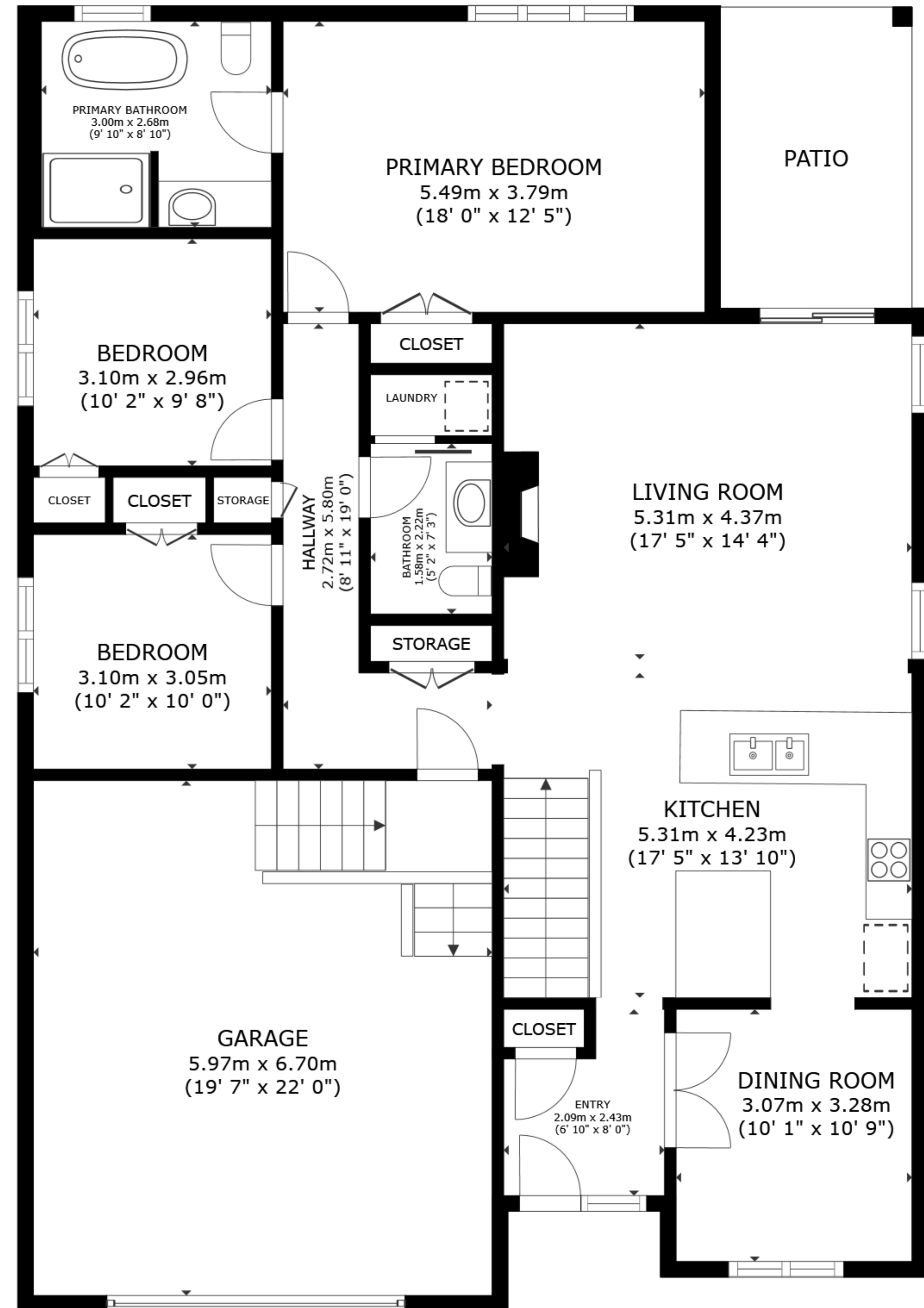
FLOOR 1
