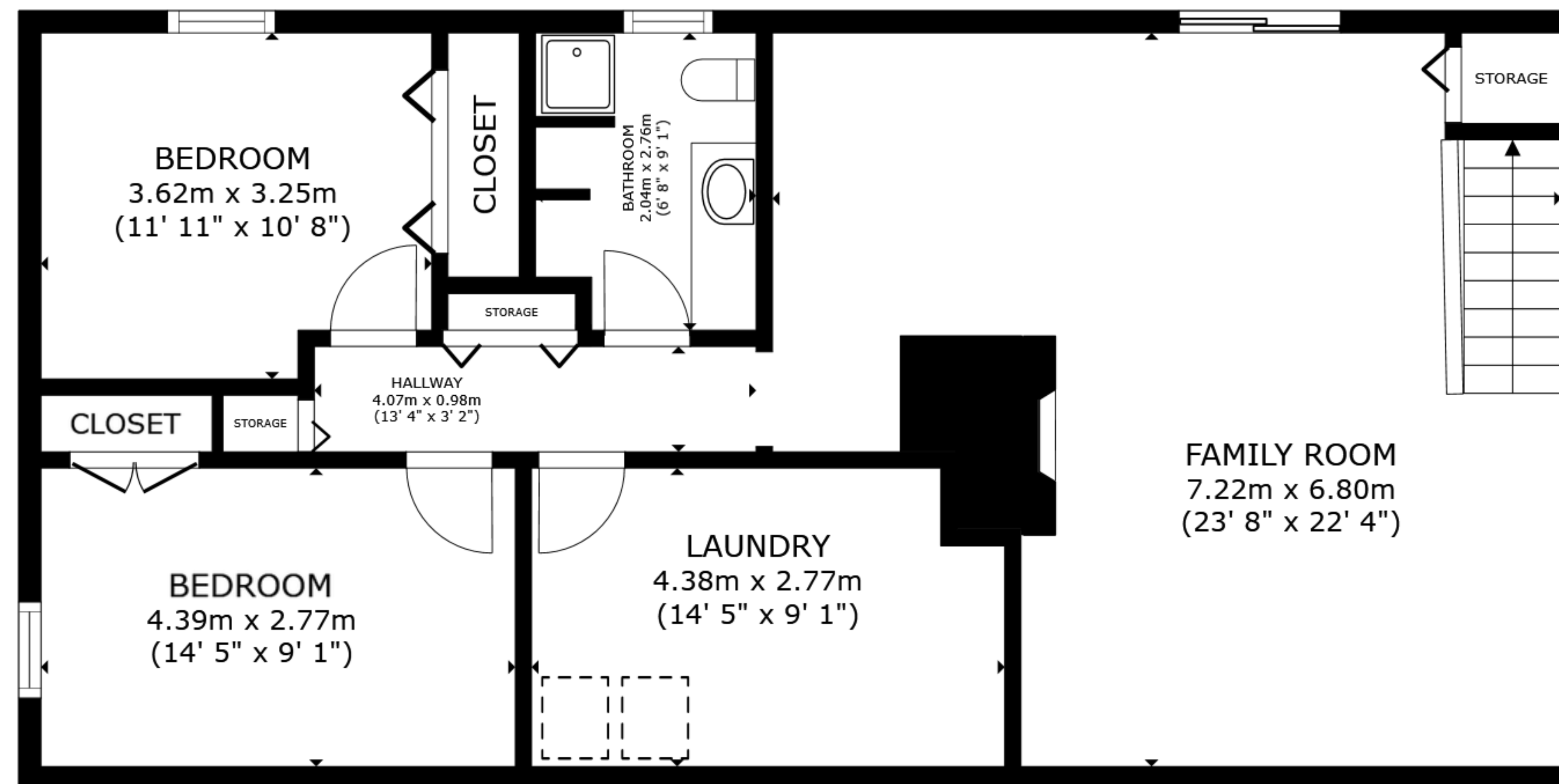
FLOOR 1
