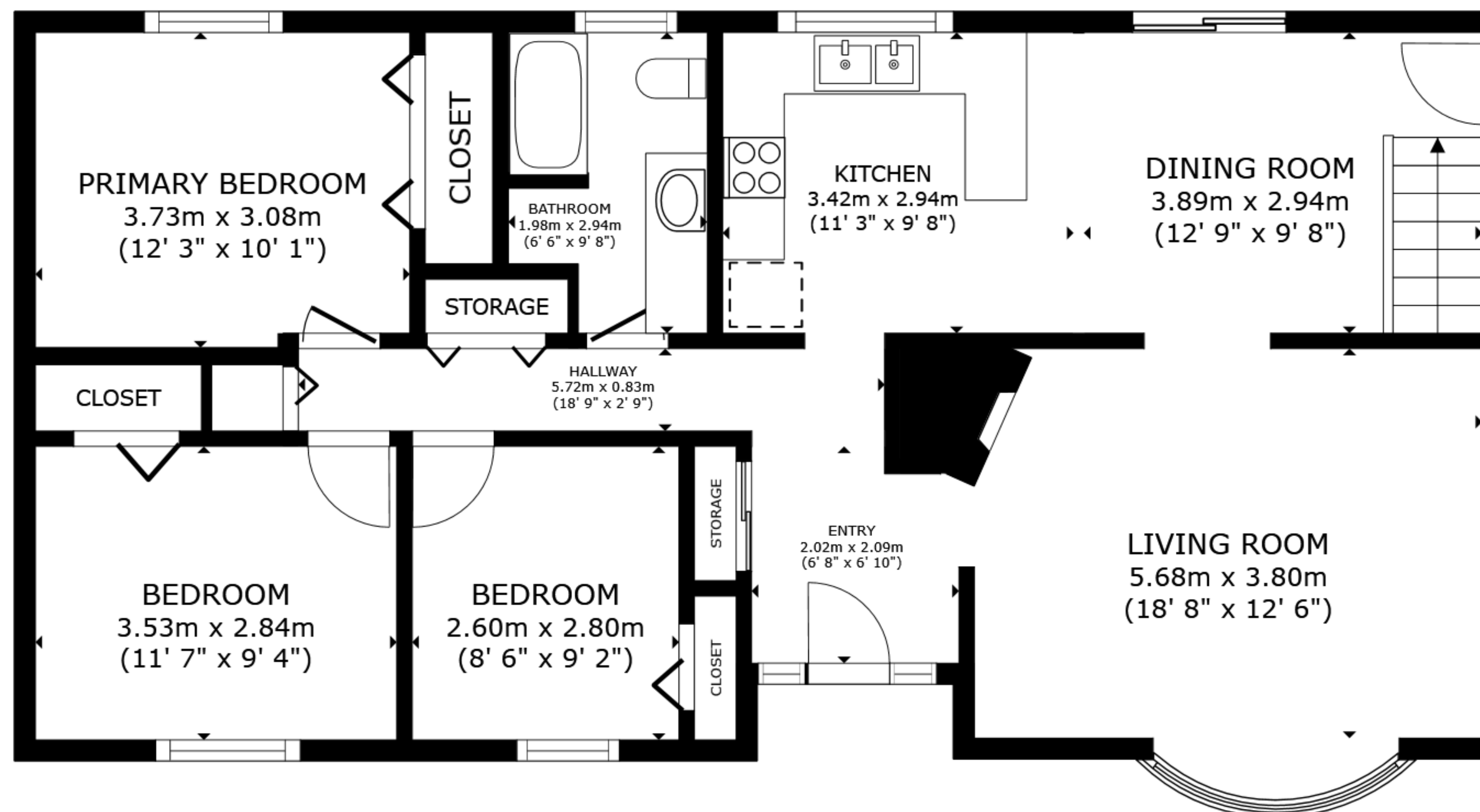
FLOOR 2
