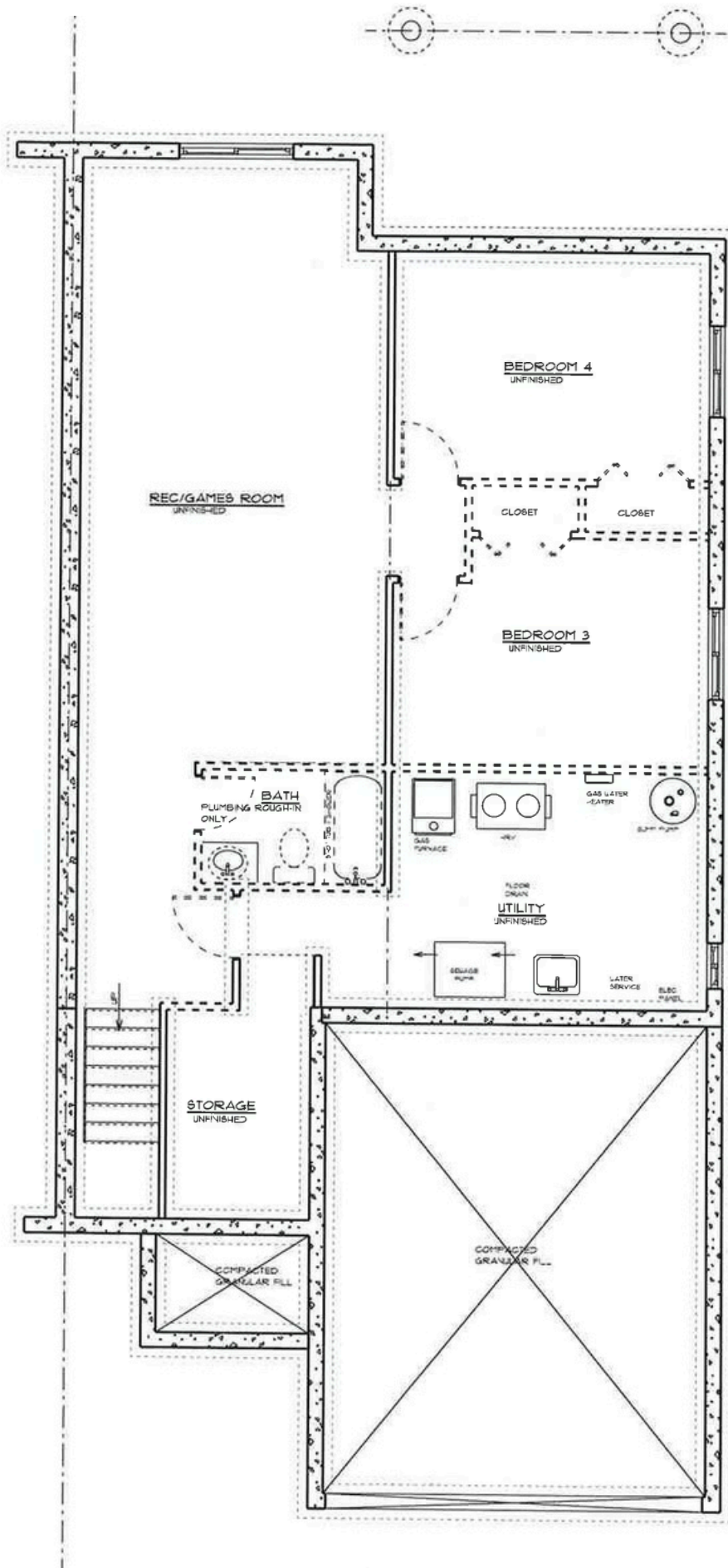
FOUNDATION PLAN VERSION B - UNFINISHED
