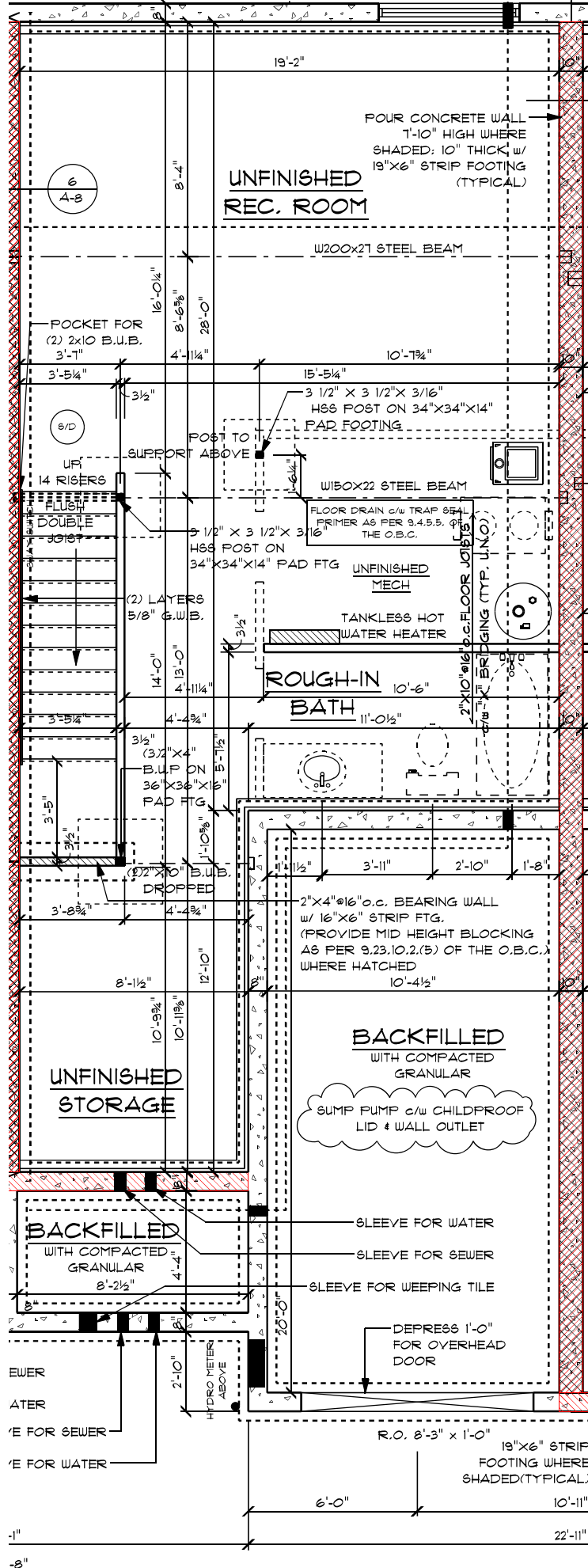
THE SYCAMORE - UNIT 46 BASEMENT PLAN
